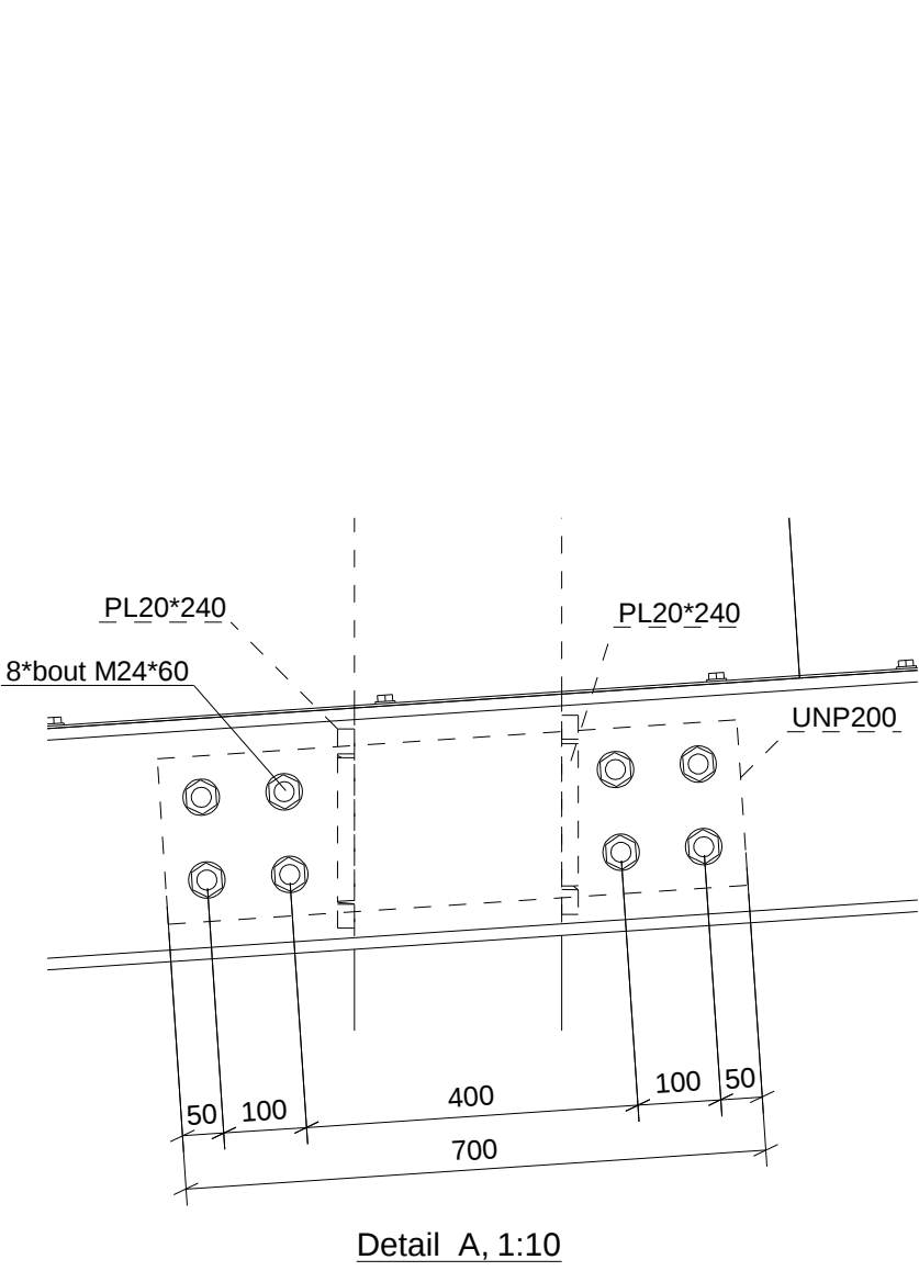
Detail A 1:10
