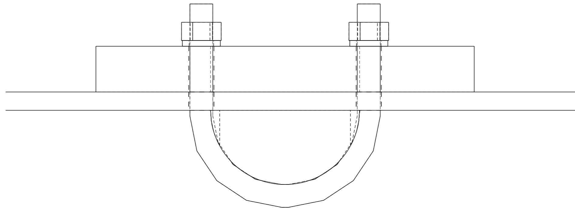
Detail beugel
